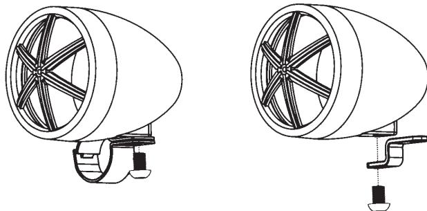
Loudspeaker mounting diagram
